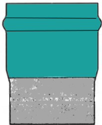
Sanded Stubs for Manholes GxS 8" Long
