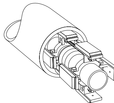
RESTRAINED CASING SPACER FOR PIPE BELL JOINT
