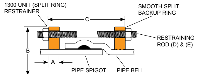
1355 ASSEMBLY
