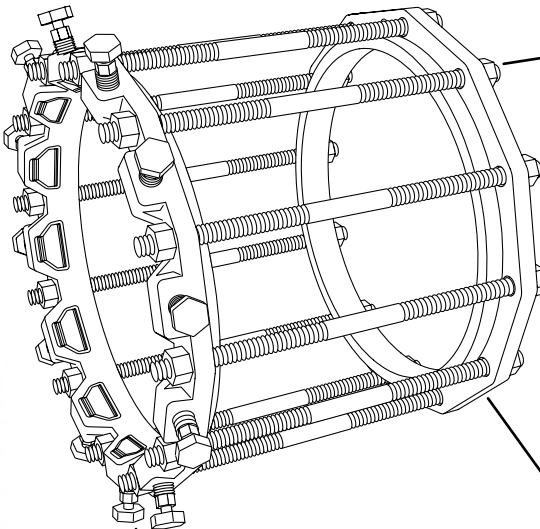
Series 1450 Installed
