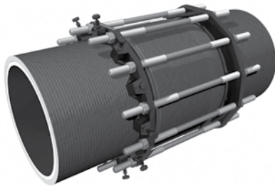
Series 1450 Installed
